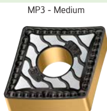
MP3 - Medium
